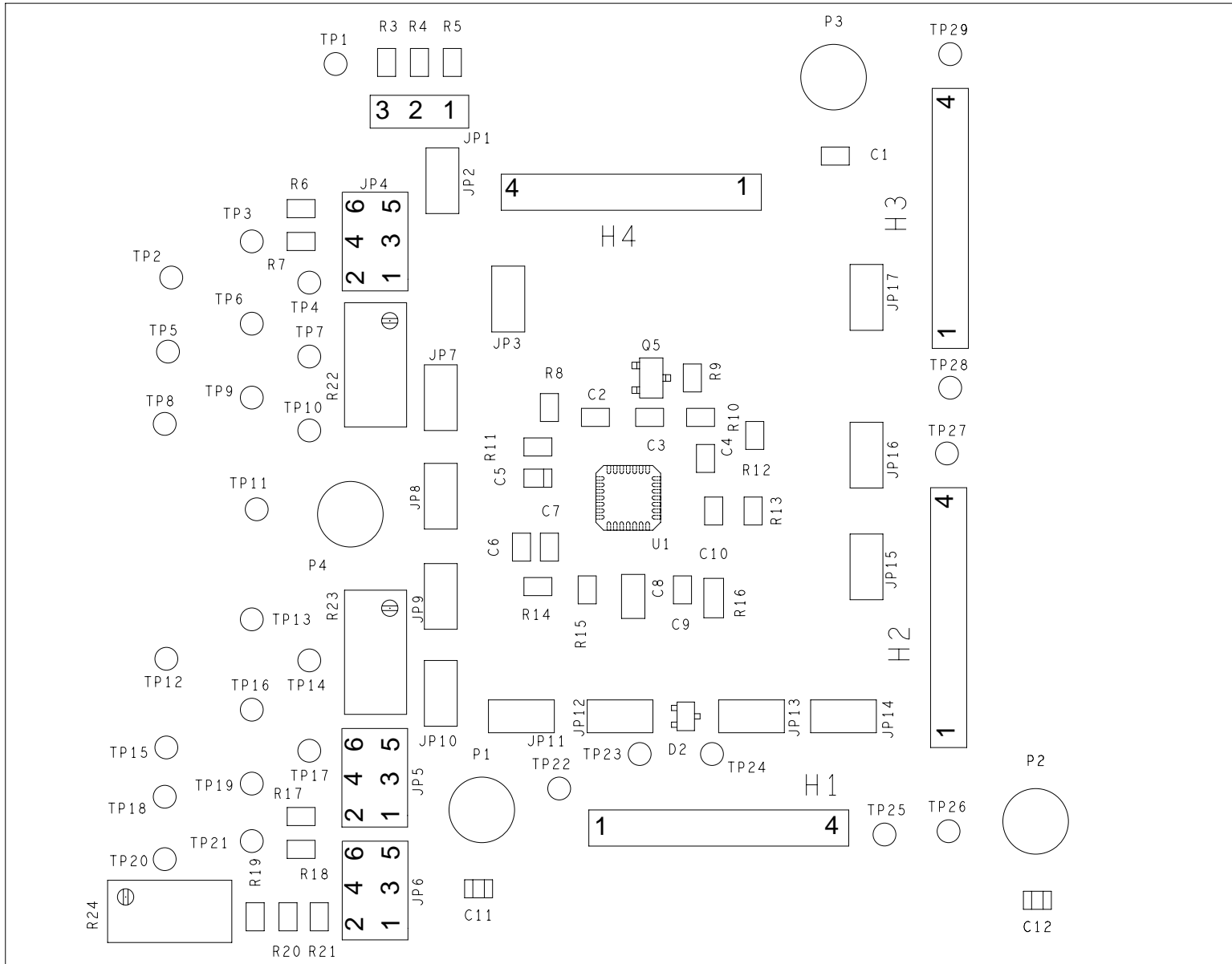
FIGURE 2. TOP SILK AND ASSEMBLY
