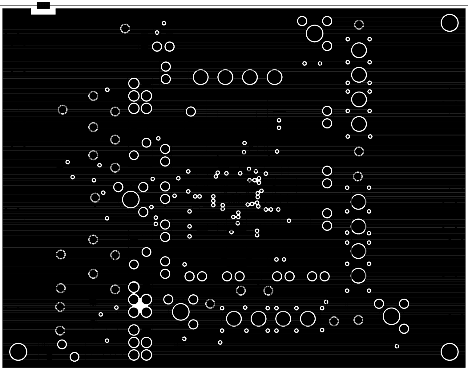
FIGURE 5. L2 GND
