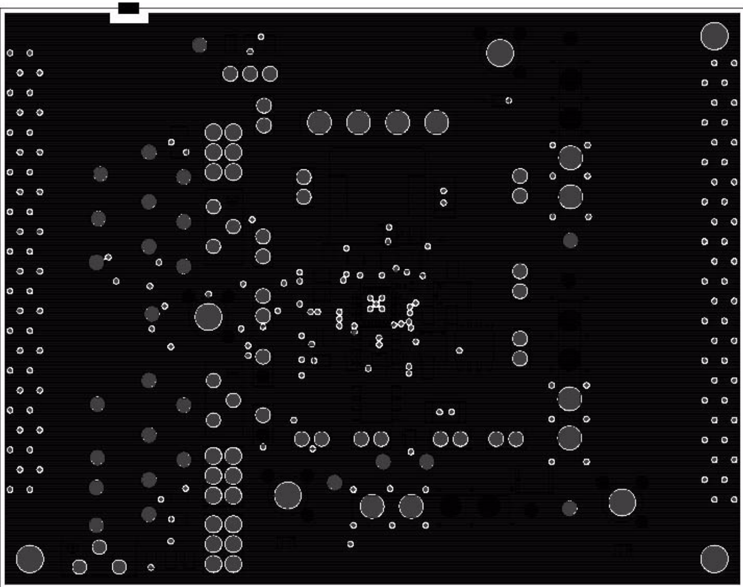
FIGURE 8. L5 GND
