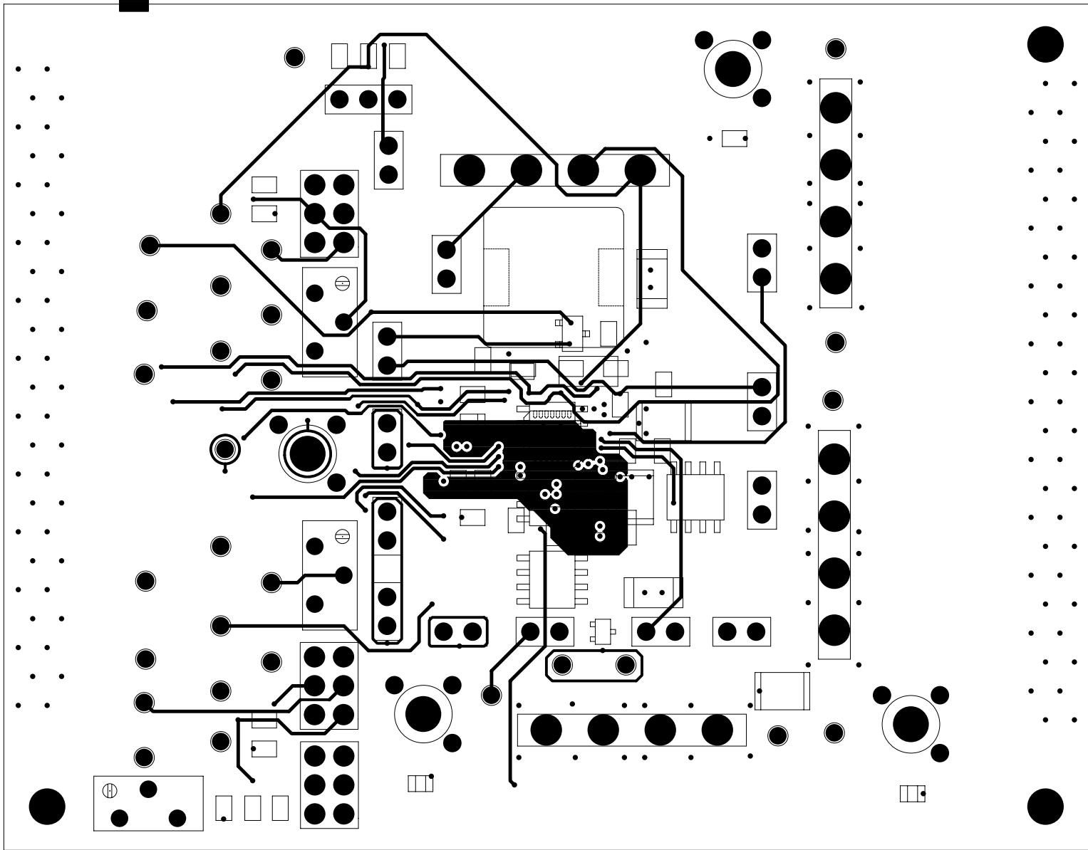
FIGURE 6. L3 SIGNAL
