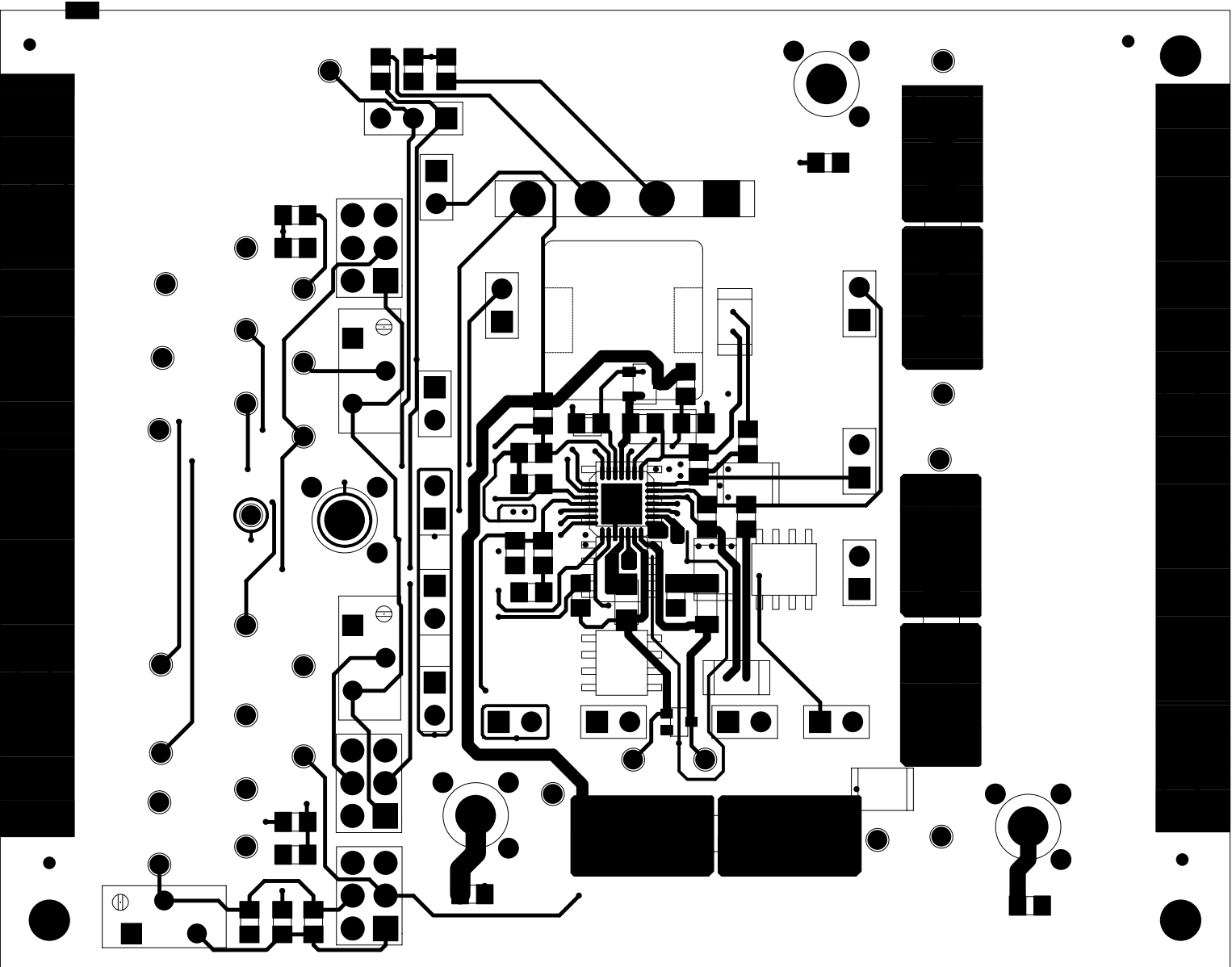
FIGURE 4. TOP
