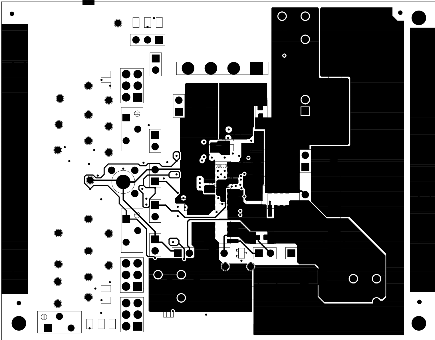
FIGURE 9. BOTTOM
