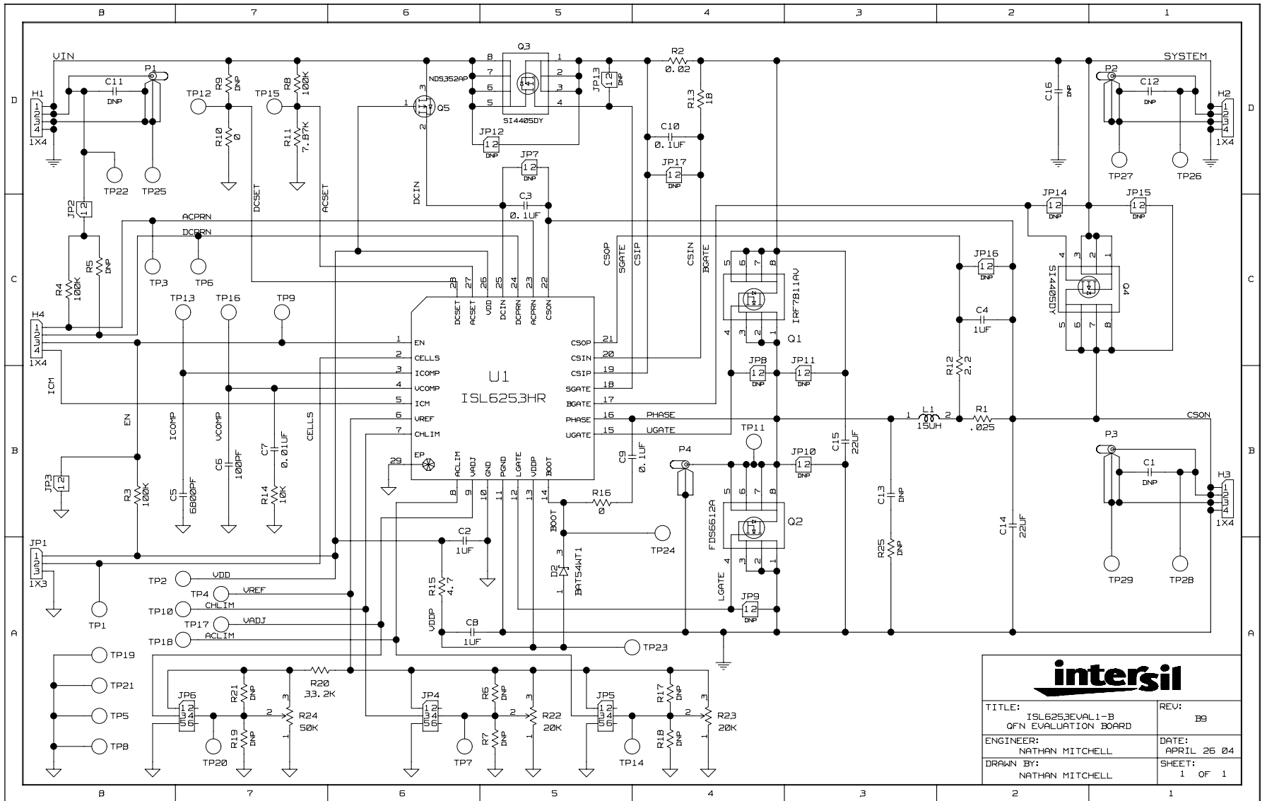
FIGURE 1. SCHEMATIC
